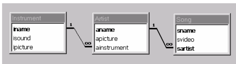
Figure 3 MMDB database
